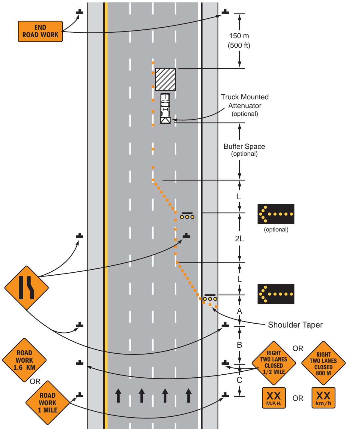
Typical Application 37
